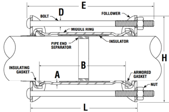
Style 39-40 Long Body Insulating Coupling
