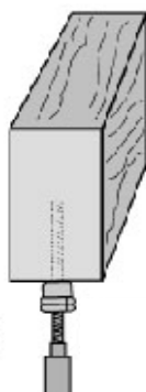
Straight Screws For 3/8" All-thread rod Min. 1/4" Steel Min. 1-1/2" Wood
