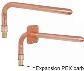
COPPER STUBOUT ELBOWS - PEX-A F1960 EXPANSION
